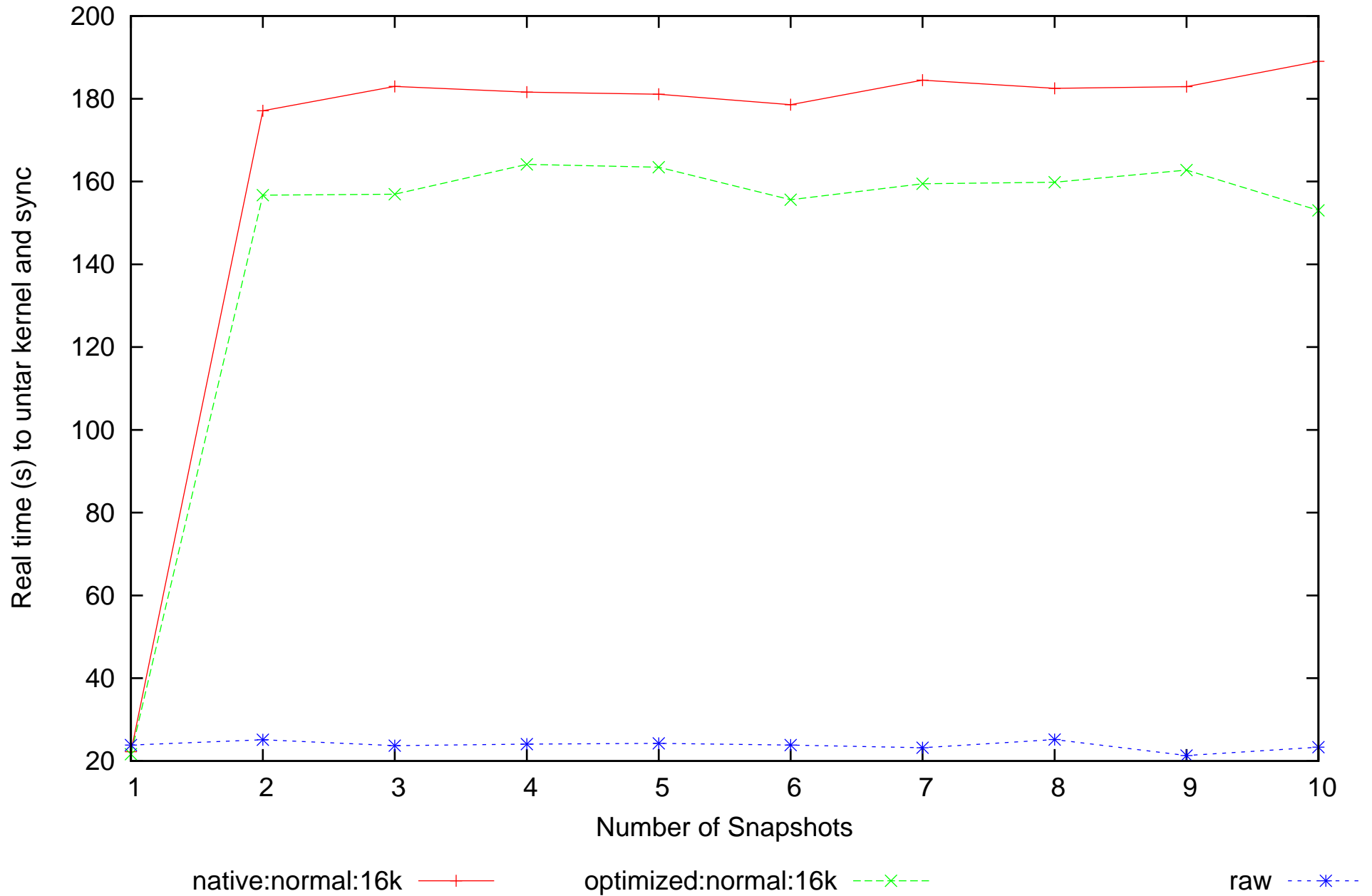
Time to untar a kernel source tree vs Number of Snapshots
