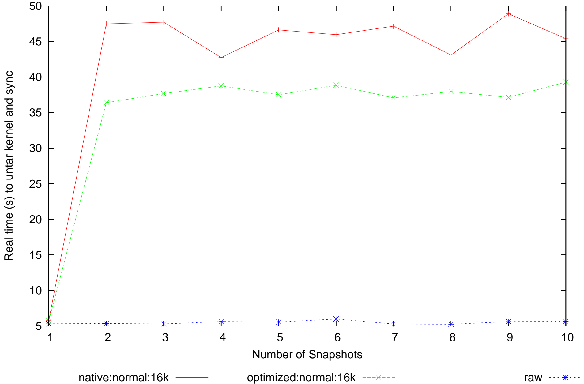
Time to untar a kernel source tree vs Number of Snapshots
