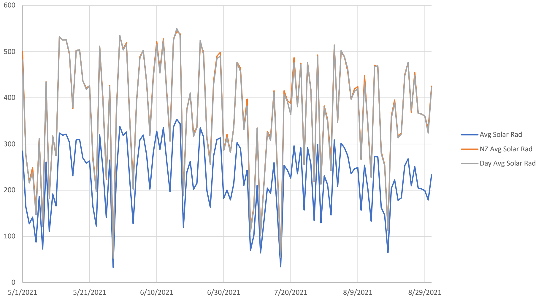
Daily Average Summer Solar Radiation Readings
