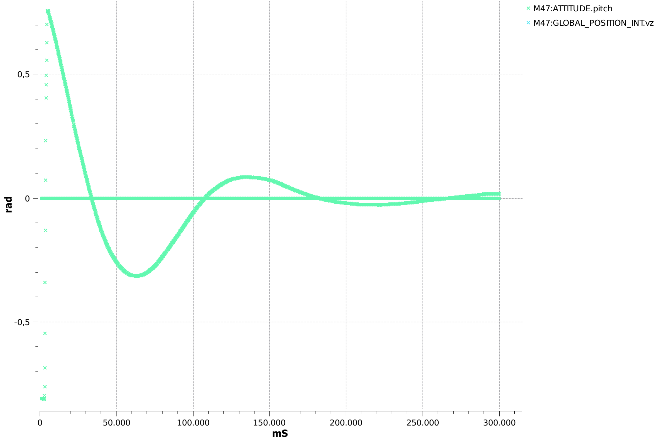
-90 to 0 after 0 -90 pitch test
