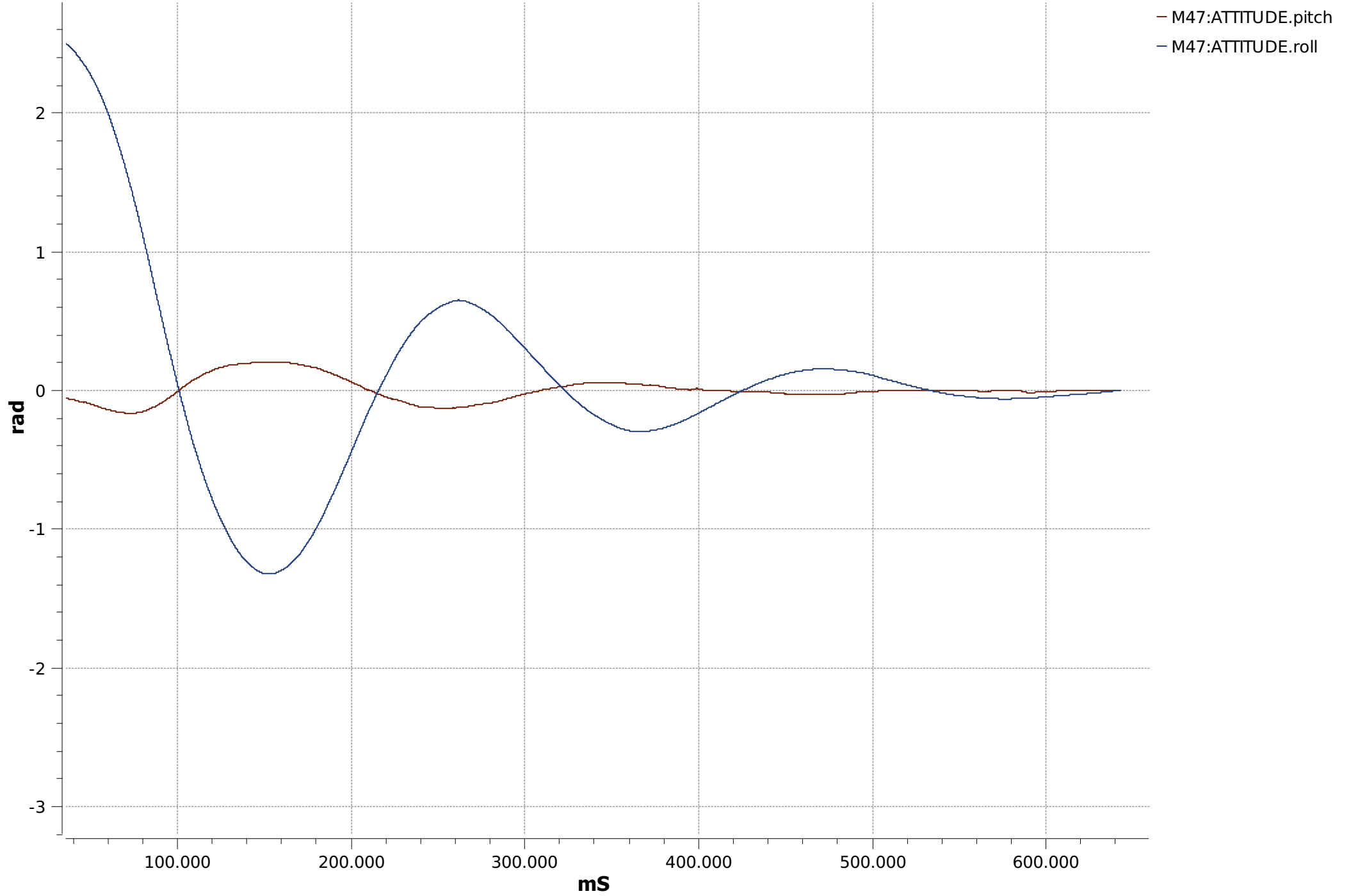
Rotation test(settling)
