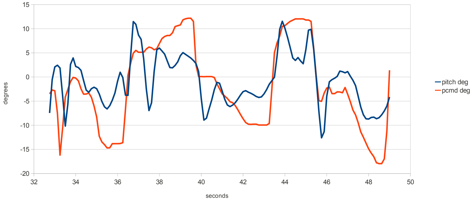
Pitch and commanded pitch
