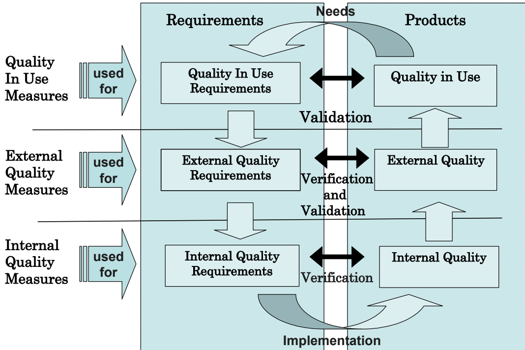
Figure 4 – Software product quality life cycle and software quality measures
