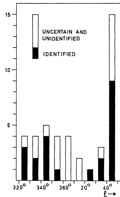
Number of sources, identified and unidentified or with uncertain identification, in 10^\circ -degree intervals in l .
