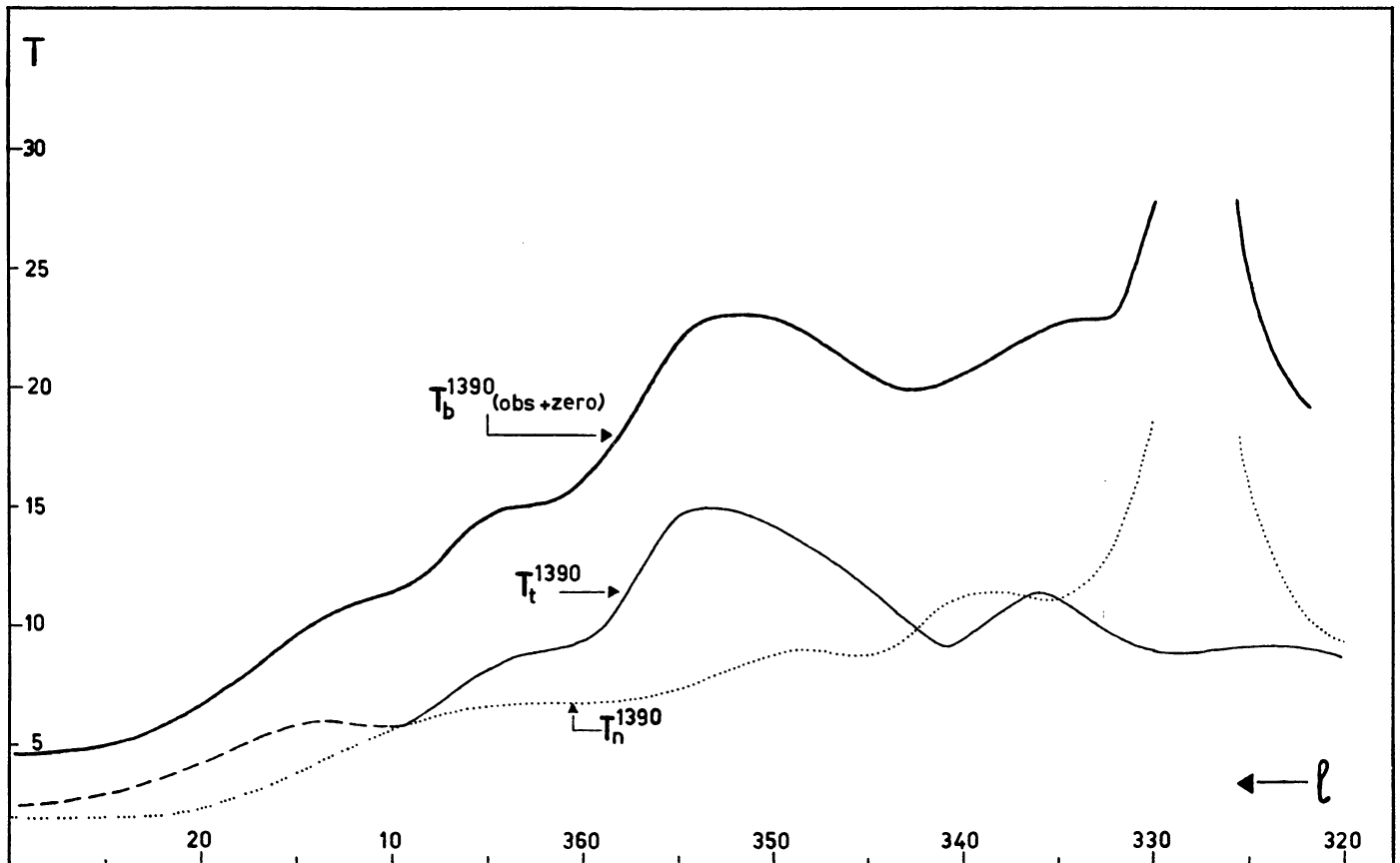
Total, thermal and nonthermal brightness temperatures along the galactic ridge, at 1390 Mc/s.
