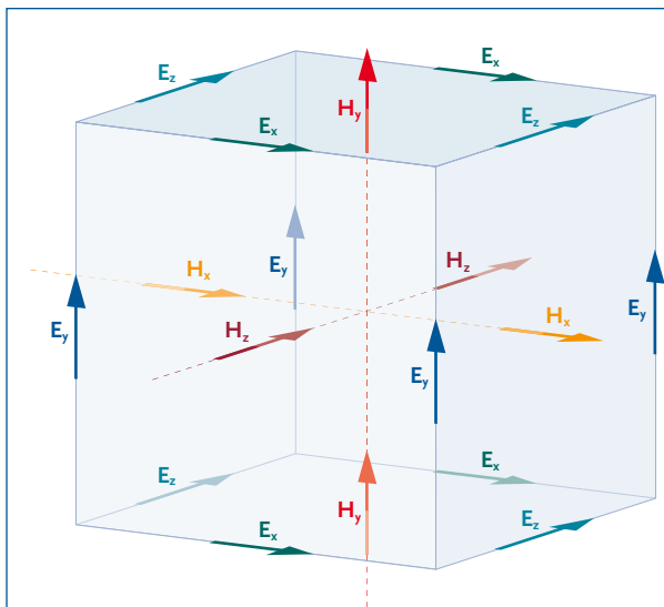
E: Electrical Field Vectors H: Magnetic Field Vectors
