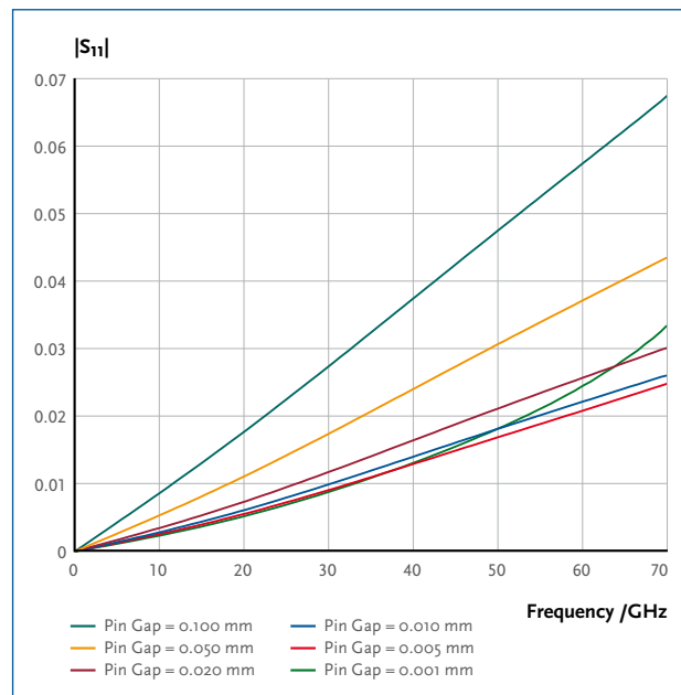
9 The same as figure 8 for a 1.85 mm connector with larger chamfers in the design of the female connector interface. The connector under consideration is not useful for metrology applications because its reflection coefficient reveals behavior close to resonance for the 0.001 mm pin gap.
