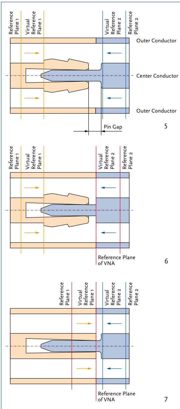
5 Longitudinal cross section of a coaxial connector with outer conductor and center conductor parts in yellow (female) and blue (male). The virtual reference planes are derived from the reference planes.
