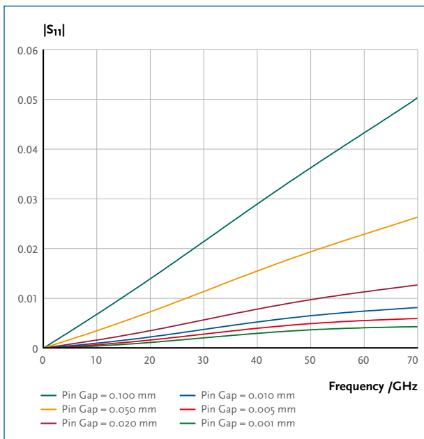
8 Absolute value of reflection coefficient of a 1.85 mm connector plotted as a function of frequency. The connector under consideration is useful for metrology applications because its reflection coefficients scale nicely with the pin gap.
