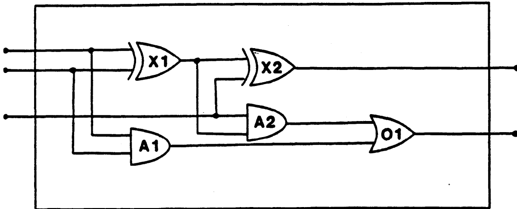
Figure 1. A full adder circuit.
