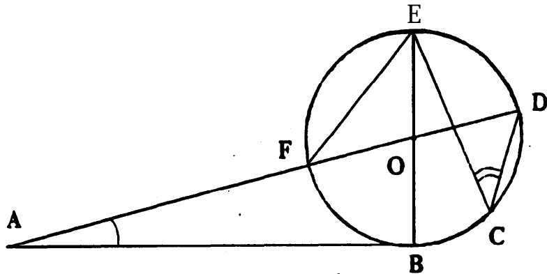
Figure 2. Given \angle OAB = 20^\circ find \angle ECD
