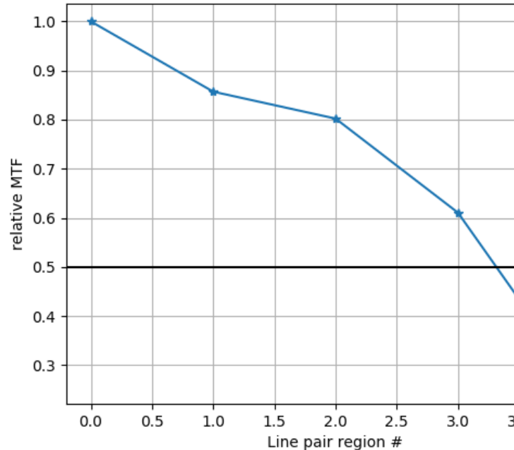
High-frequency rMTF
