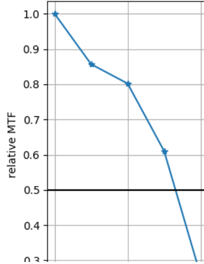
High-frequency rMTF
