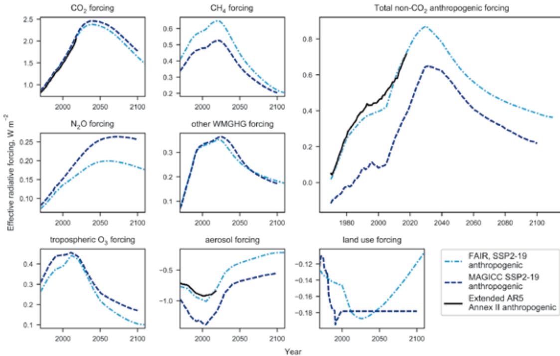
Figure 2.SM.2 | Time series of MAGICCC (dark blue dashed) and FAIR (sky blue dash-dotted) effective radiative forcing for an example emission scenario for the main forcing agents where the models exhibit differences. AR5 data is from Myhre et al. (2013), extended from 2011 until the end of 2017 with greenhouse gas data from NOAA/ESRL ( www.esrl.noaa.gov/gmd/ccgg/trends/ ), updated radiative forcing approximations for greenhouse gases (Etminan et al., 2016) and extended aerosol forcing following (Myhre et al., 2017).
