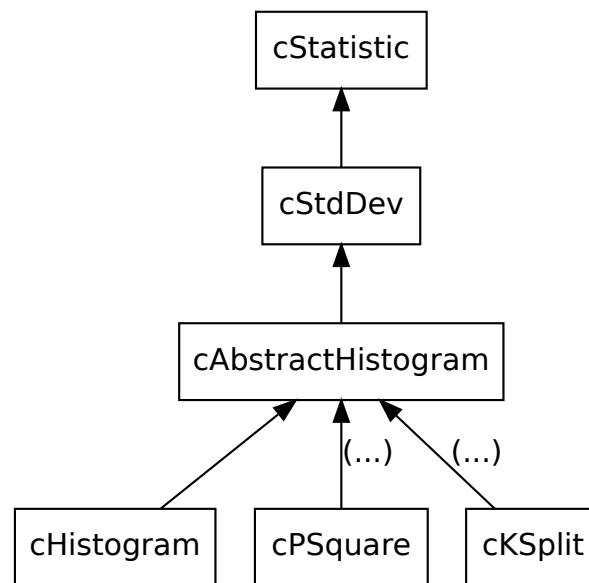
Figure 7.4: Statistics classes
