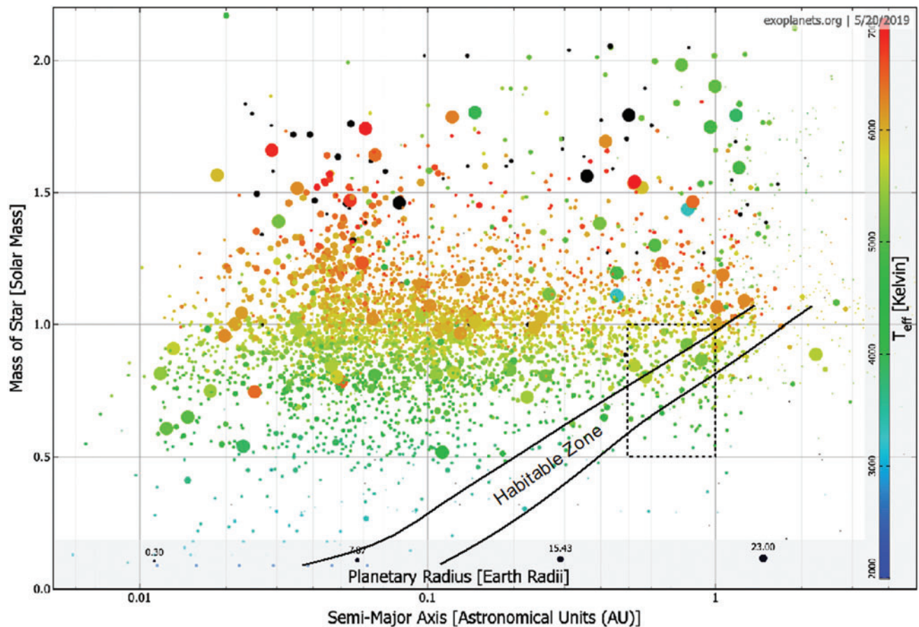
FIG. 1. Star-planet distances (along the abscissa) and mass of the host star (along the ordinate) of roughly 4500 extrasolar planet and extrasolar planet candidates. The temperatures of the stars are indicated with symbol colors (see color bar). Planetary radii are encoded in the symbol sizes (see size scale at the bottom). The conservative habitable zone, defined by the moist-greenhouse and the maximum greenhouse limits (Kopparapu et al. , 2013) is outlined with black solid lines. Stellar luminosities required for the parameterization of these limits were taken from Baraffe et al. (2015) as a function of mass as shown along the ordinate of the diagram. The dashed box refers to the region shown in Fig. 2. Data from exoplanets.org as of May 20, 2019. Color images are available online.
