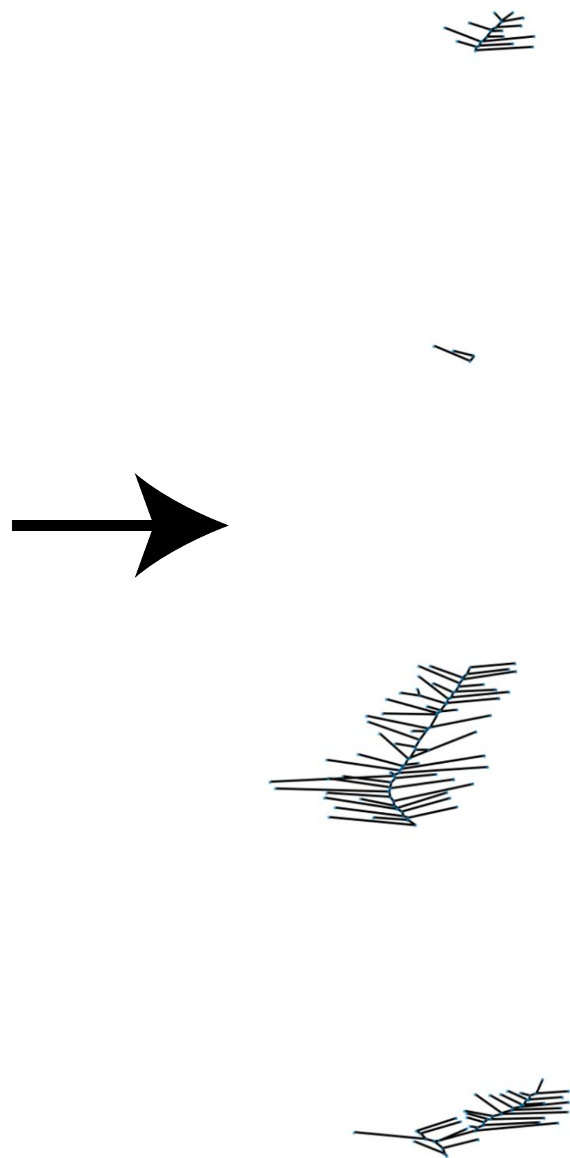
Networkx subgraphs
