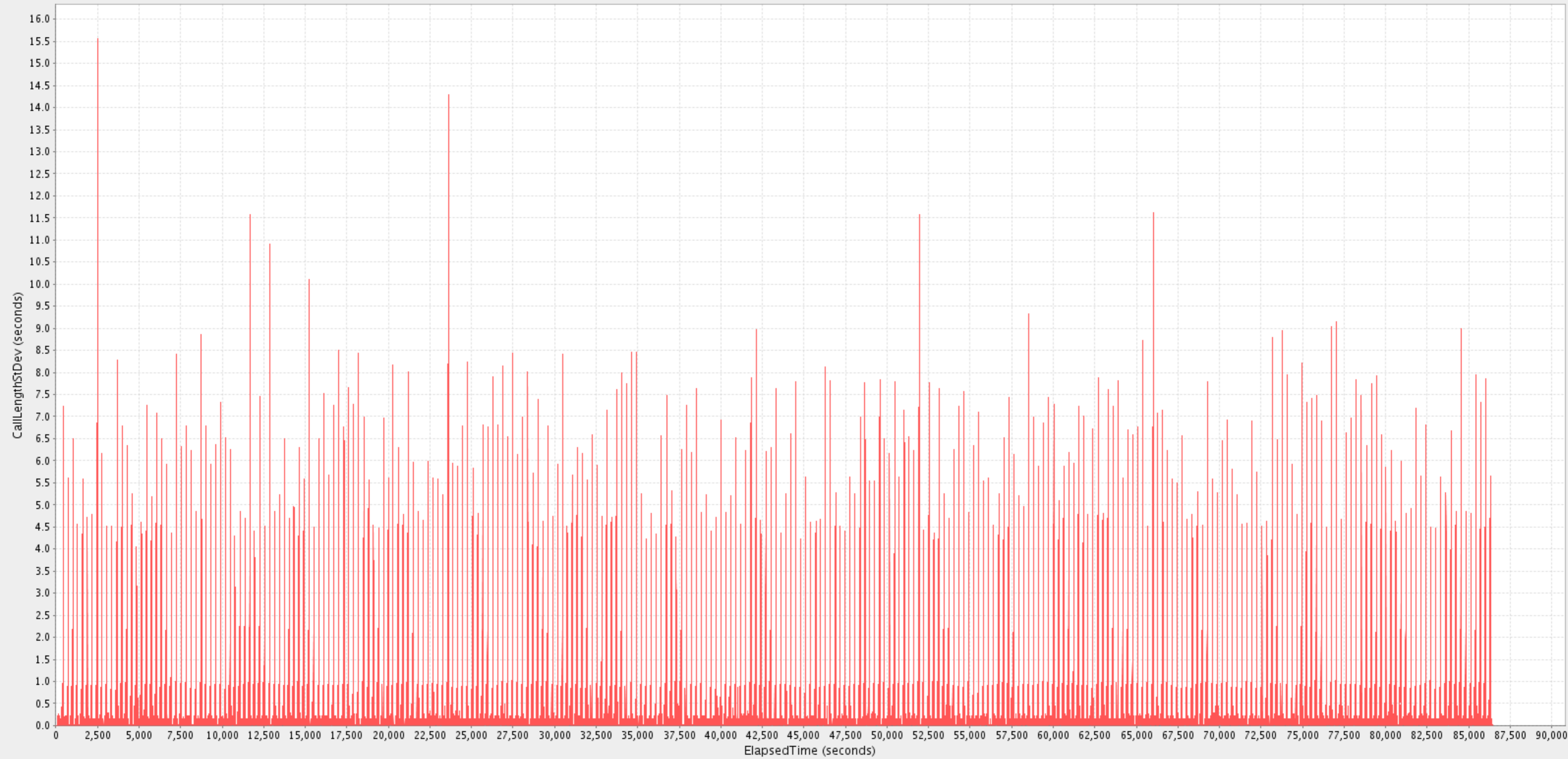
CallLengthStDev (Periodic)
