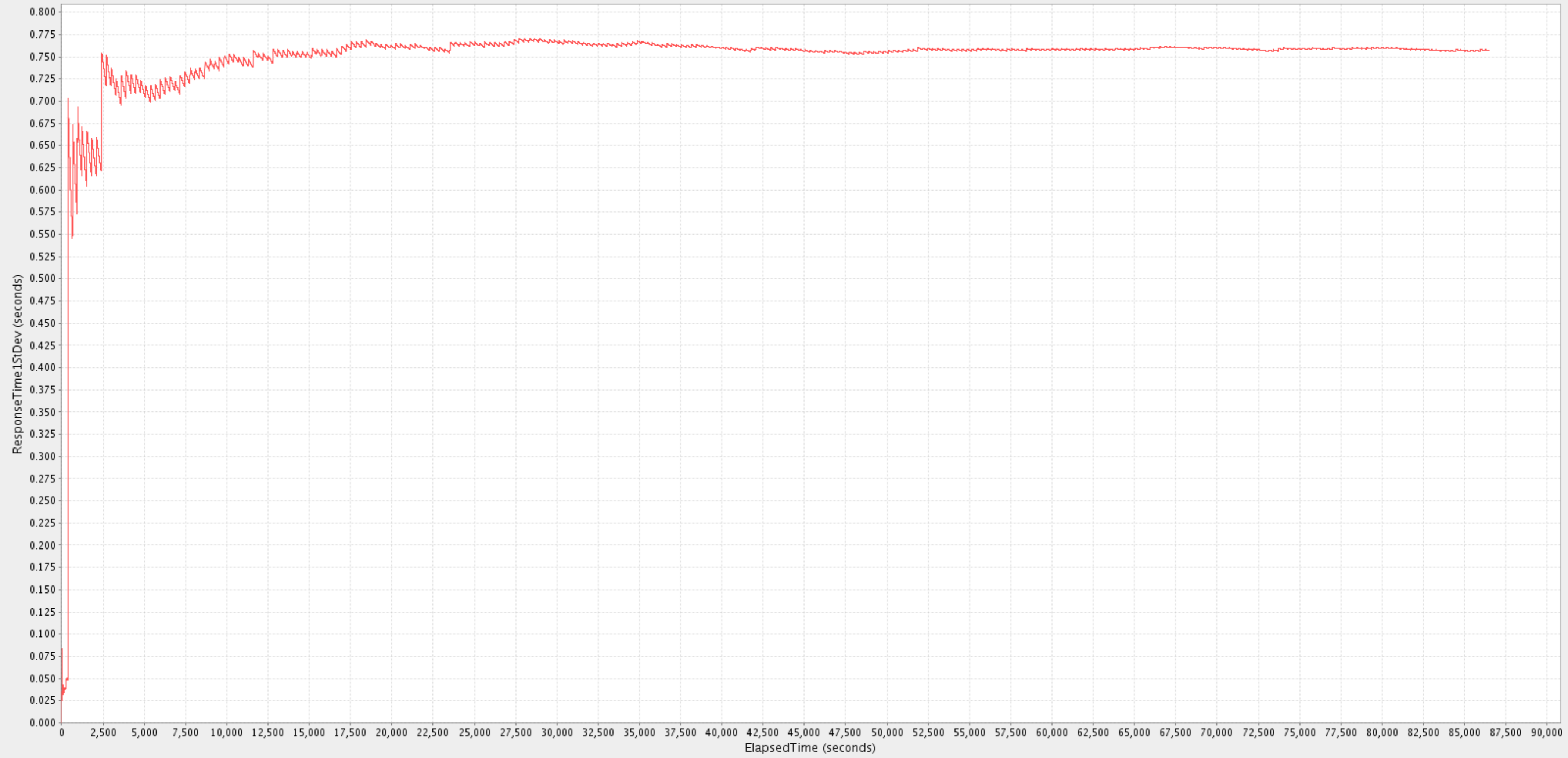
ResponseTime1StDev (Average)
