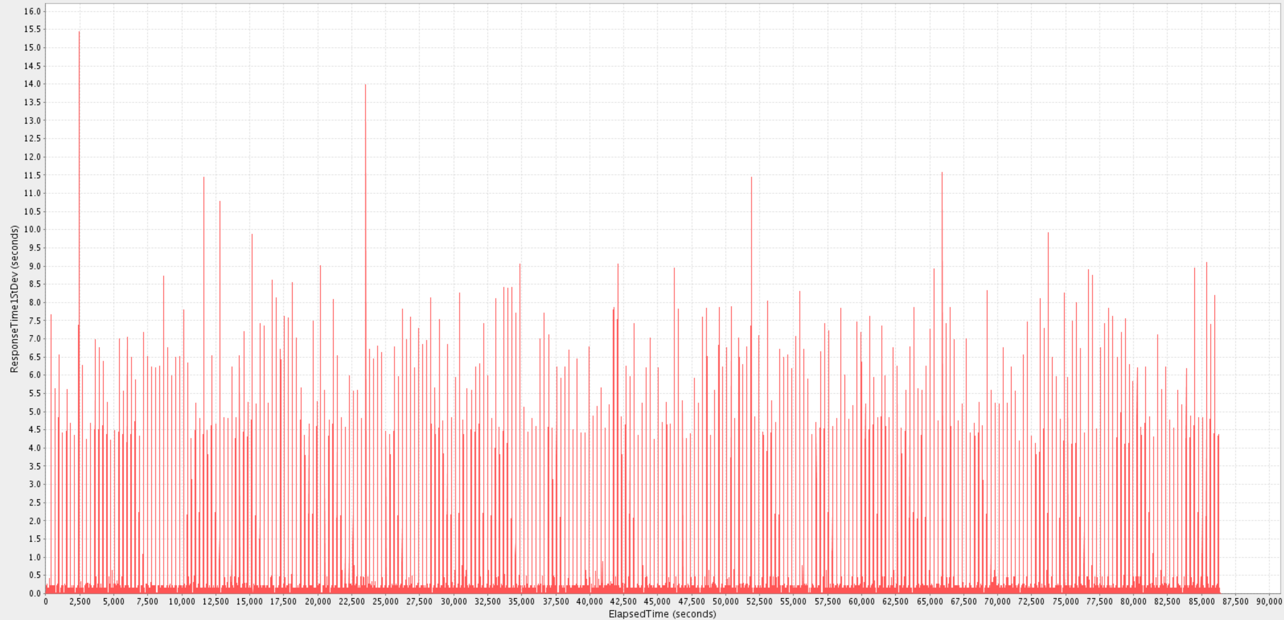
ResponseTime1StDev (Periodic)
