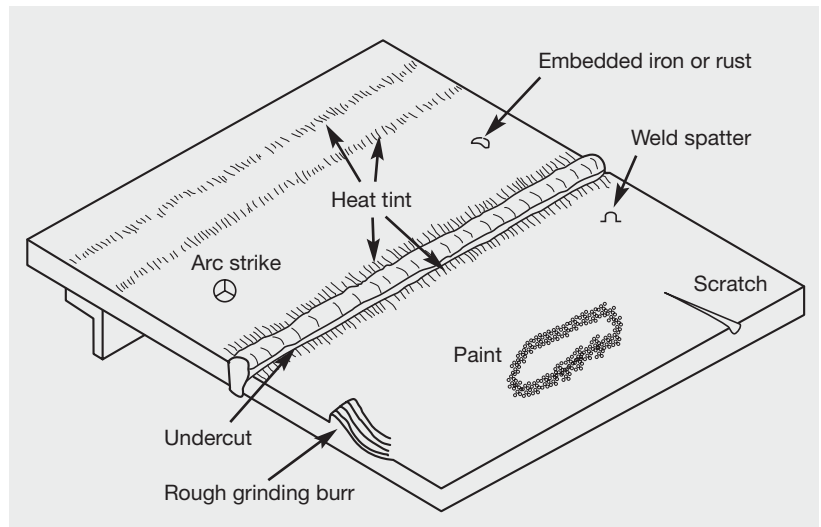
Figure 18. Typical fabrication defects or surface conditions which may be encountered (Source: Nickel Institute Publication 10 026)
