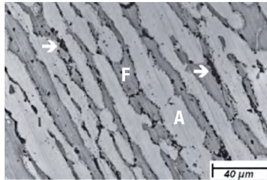
Figure 4: Microstructure of a 2205 sample aged at 850°C (1560°F) for 40 minutes showing sigma phase precipitation (arrows) on the austenite/ferrite grain boundaries. The ferrite (F) phase appears darker than the austenite (A) phase in the micrograph (Ref. 3).
