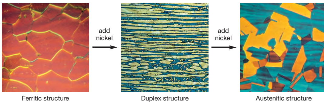
Figure 2: Increasing the nickel content changes the microstructure of a stainless steel from ferritic (left) to duplex (middle) to austenitic (right) (These pictures, courtesy of Outokumpu, show polished and etched samples, enlarged under a light microscope. In the duplex structure, the ferrite has been stained so that it appears as the darker phase.)
