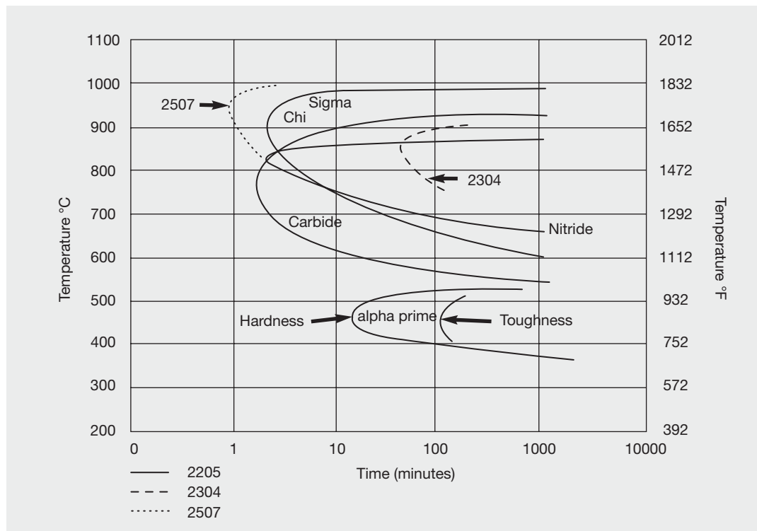
Figure 5: Isothermal precipitation diagram for 2205 duplex stainless steel, annealed at 1050°C (1920°F). (Duplex grades 2304 and 2507 are shown for comparison)
