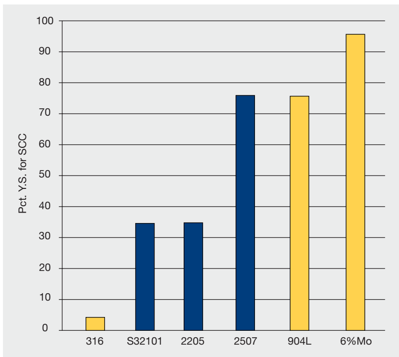
Figure 9: Stress corrosion cracking resistance of mill annealed austenitic and duplex stainless steels in the drop evaporation test with sodium chloride solutions at 120°C (248°F) (stress that caused cracking shown as a percentage of yield strength) (Source: Outokumpu).
