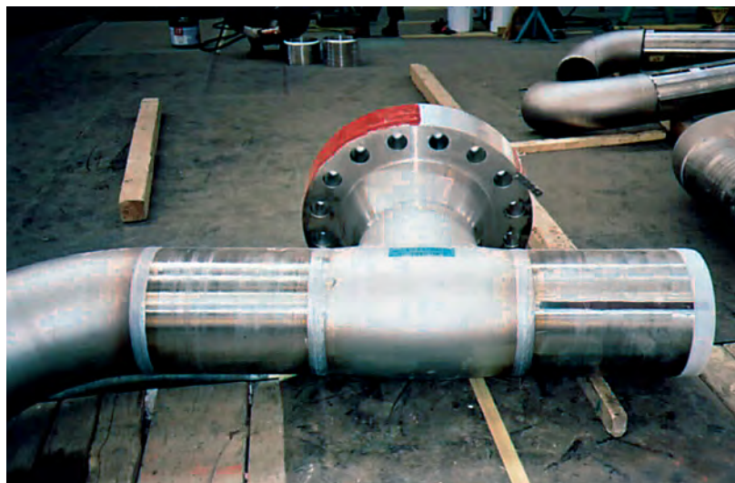
2205 Flanged T-piece (Source: Arco Exploration and Production Technology)
