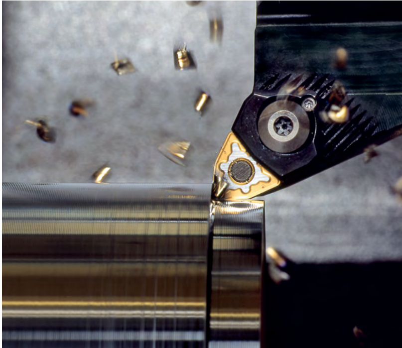
Turning operation (Source: Seco Tools)
