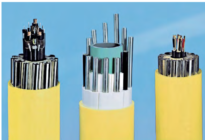
2507 umbilical tubing for offshore oil and gas applications (Source: Sandvik)
