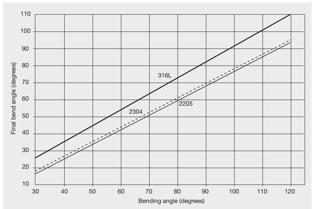
Figure 12. Comparison of springback of duplex stainless steels and type 316L for 2 mm (0.08 inch) thick sheet (Source: Outokumpu)
