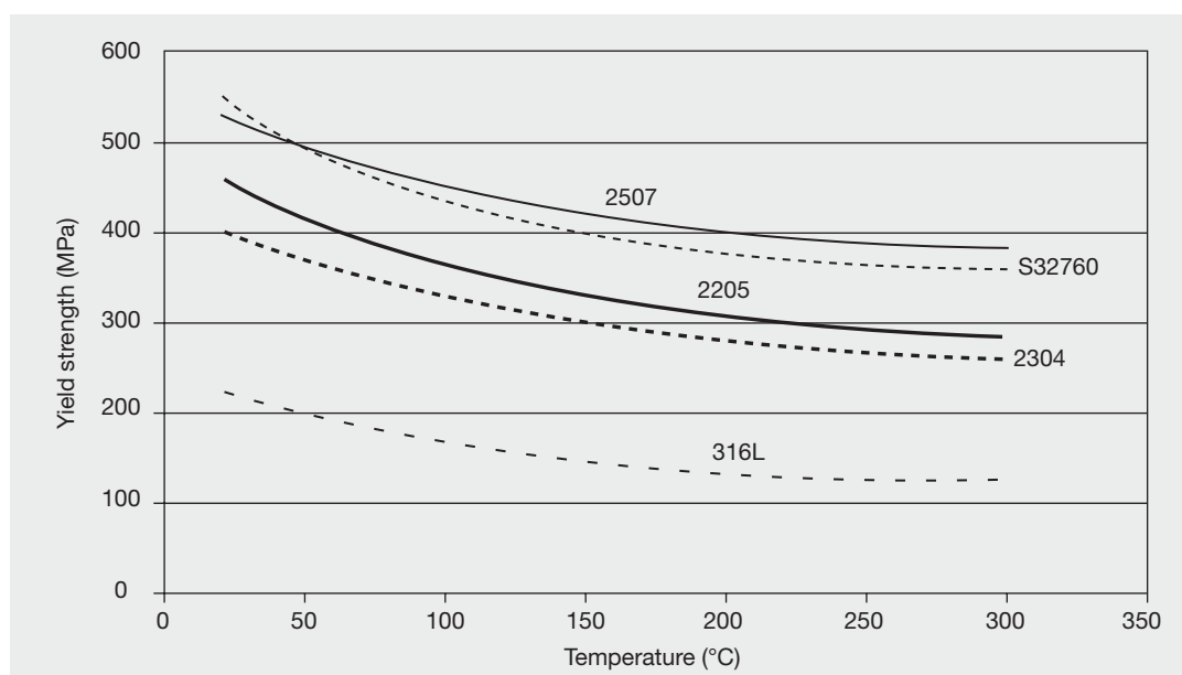
Figure 11: Comparison of typical yield strength of duplex stainless steels and Type 316L between room temperature and 300°C (572°F) (Source: producer data sheets)
