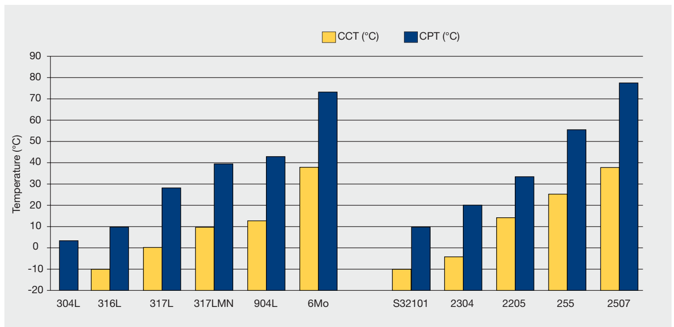
Figure 8: Critical pitting and crevice corrosion temperatures for unwelded austenitic stainless steels (left side) and duplex stainless steels (right side) in the solution annealed condition (evaluated in 6% ferric chloride by ASTM G 48)
