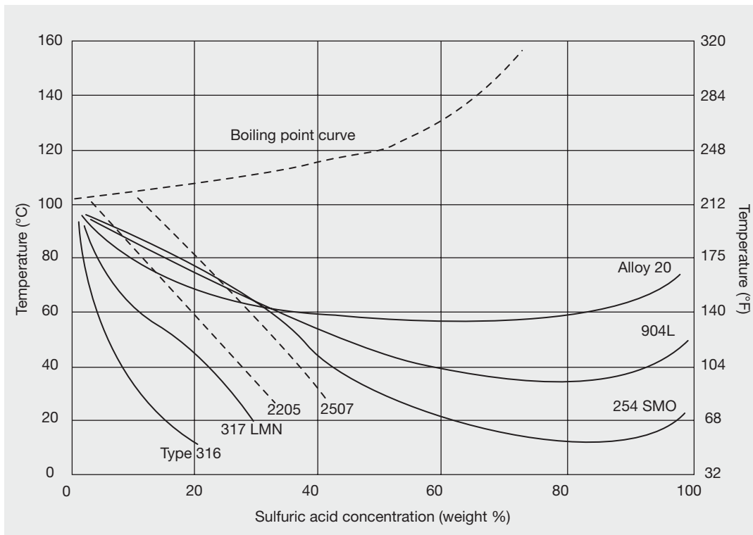
Figure 6: Corrosion in non-aerated sulfuric acid, 0.1 mm/yr (0.004 inch/yr) isocorrosion diagram (laboratory tests using reagent grade sulfuric acid). (Source: Producer data sheets, 254 SMO is a trademark of Outokumpu)
