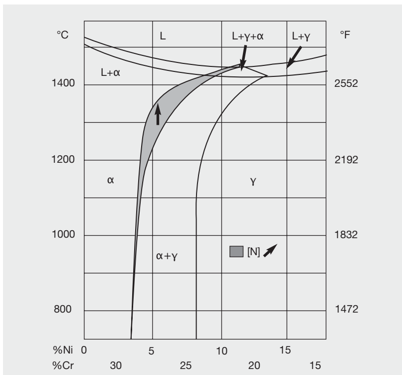
Figure 3: Section through the Fe-Cr-Ni ternary phase diagram at 68% iron (small changes in the nickel and chromium content have a large influence on the amount of austenite and ferrite in duplex stainless steels.)
