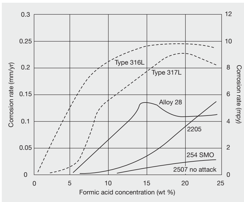
Figure 7: Corrosion of duplex and austenitic stainless steels in boiling mixtures of 50% acetic acid and varying proportions of formic acid (Source: Sandvik)
