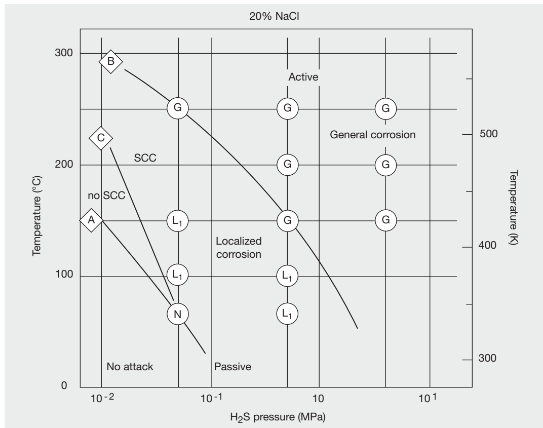
Figure 10: Corrosion of 2205 duplex stainless steel in 20% sodium chloride-hydrogen sulfide environments based on electrochemical prediction and experimental results.
