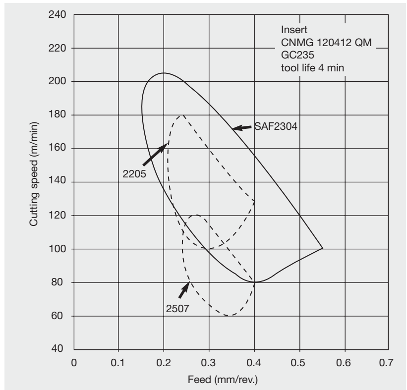
Figure 16: Comparison of machining parameters for turning duplex stainless steels with a cemented carbide insert with a tool life of four minutes (Source: Sandvik)
