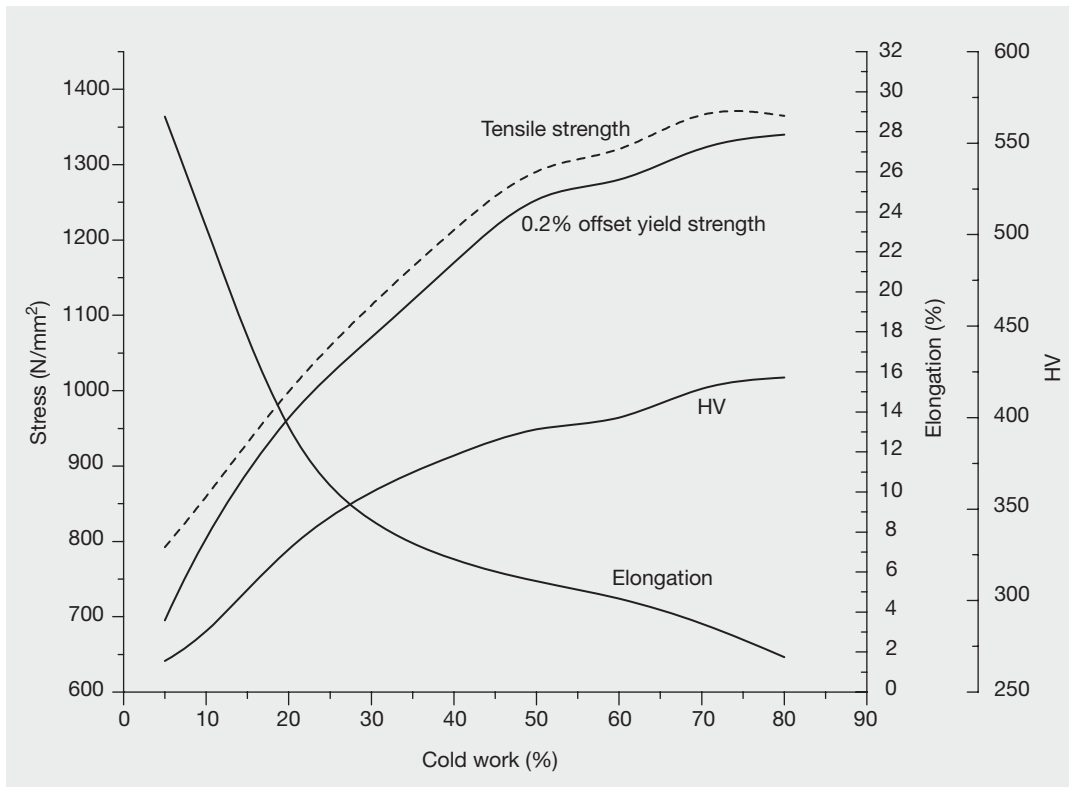
Figure 13. Effect of cold work on the mechanical properties of 2205 duplex stainless steel (Source: Baosteel)
