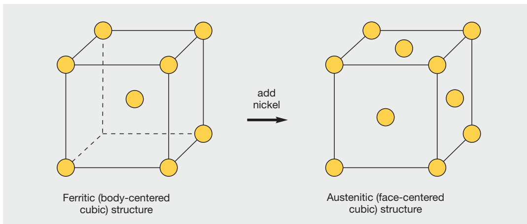
Figure 1: By adding nickel, the crystallographic structure changes from body-centered cubic (little or no nickel) to face-centered cubic (at least 6% nickel – 300 series). The duplex stainless steels, with their intermediate nickel content, have a microstructure in which some grains are ferritic and some are austenitic, ideally, about equal amounts of each (Figure 2).
