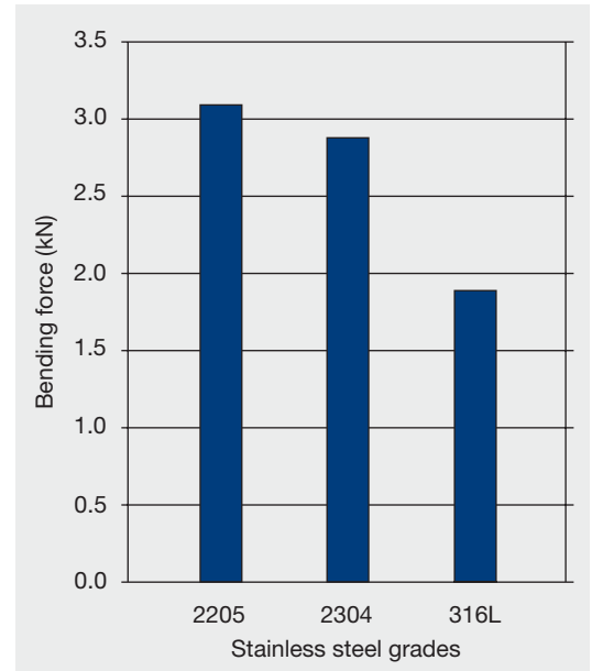
Figure 14: Minimum force required to begin plastic deformation in bending of 2304, 2205, and 316L test samples 50 mm (2 inch) wide and 2 mm (0.08 inch) thick (Source: Outokumpu)
