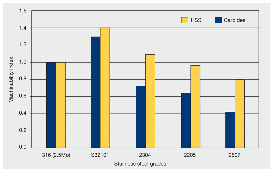
Figure 15. Relative machinability of duplex stainless steels compared with Type 316 (2.5Mo) for cemented carbide tooling and for high speed steel tooling (Source: Outokumpu)
