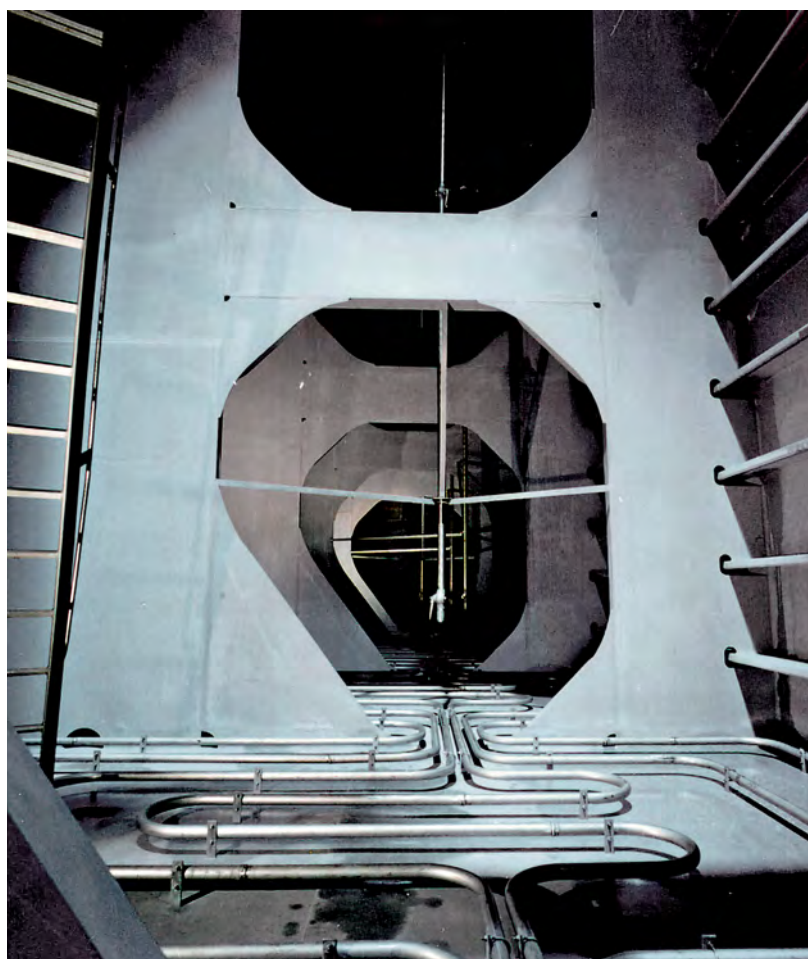
Inside a 2205 (1.4462) tank on a marine chemical tanker (Source: ThyssenKrupp Nirosta)
