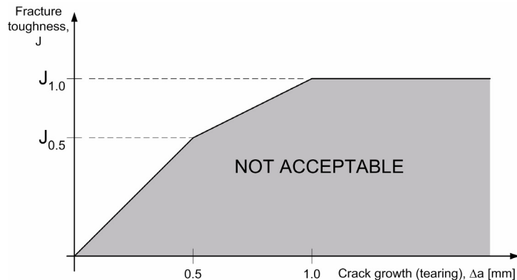
Figure 3 No J Δa test results shall end-up inside the area indicated
