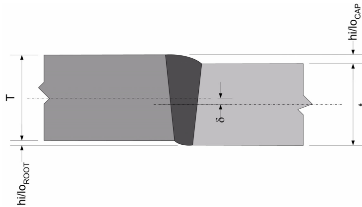
Figure 4 Illustration of how the maximum SCF may be assumed
