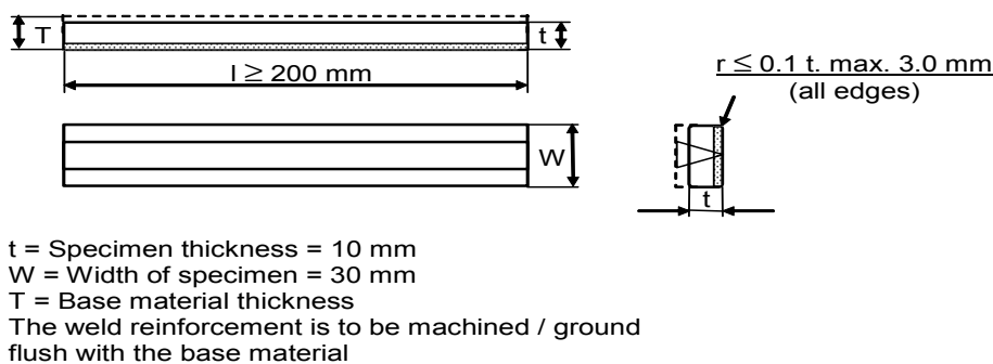
Figure 2 Longitudinal root bend test specimens
