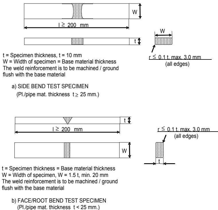
Figure 1 Bend test specimens
