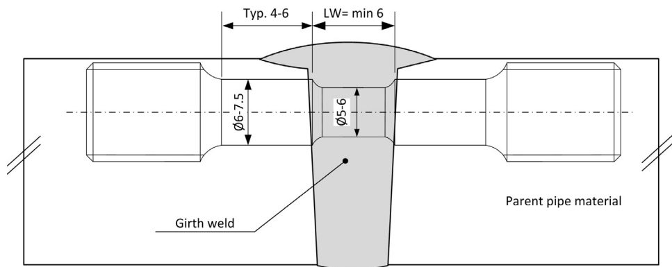
Figure 13 Tensile specimen for determination of stress/strain curves of weld metals in the weld transverse direction
