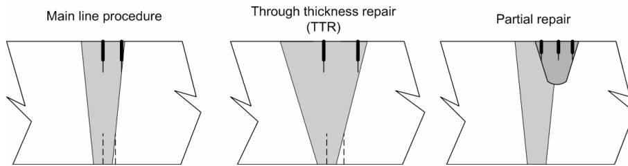
Figure 9 Illustration of typical notch positions for fracture toughness testing of girth welds
