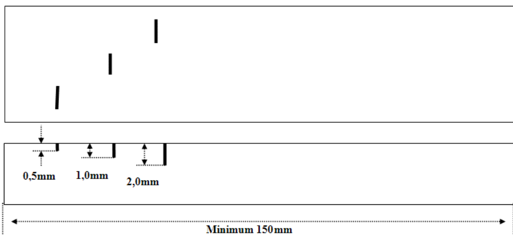
Figure 3 Reference block for sensitivity setting for creep wave probes, dimensions
