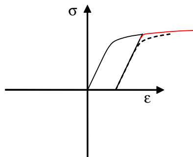
Figure 7 Cyclic strain hardening is the effect seen if a material is strained in one direction followed by unloading before the material is strained in the same direction once more. The effect of such cycling is that the yield stress is increased and that the strain-hardening is decreased
