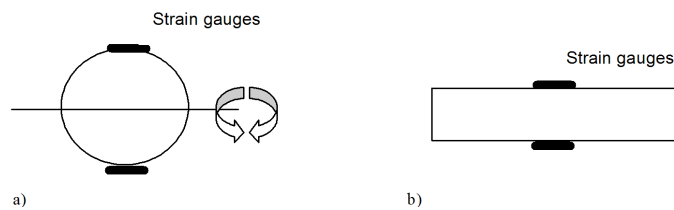
Figure 14 Instrumentation of pipe section of samples for pre-straining of materials
