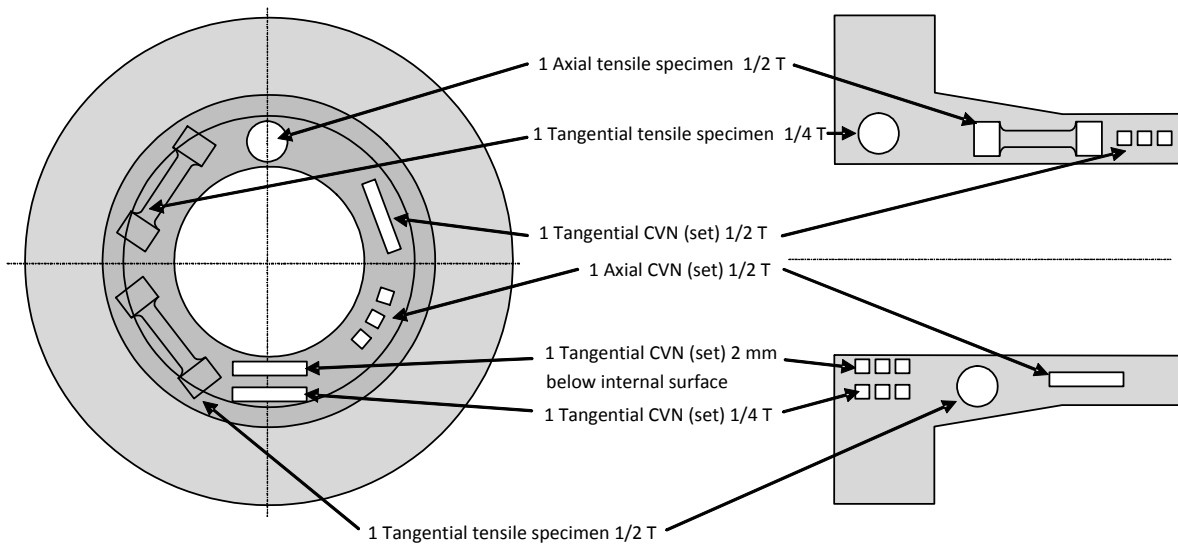
Figure 1 Location of tensile and CVN specimens, component with section thickness ≥ 25 mm
