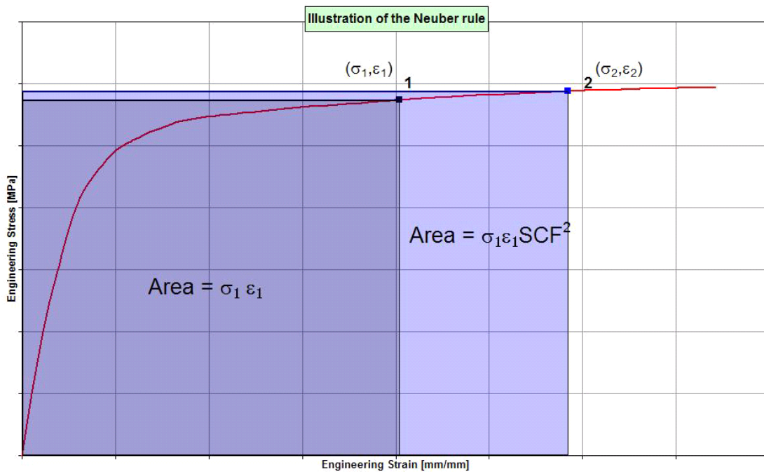
Figure 5 Illustration of the Neuber rule
