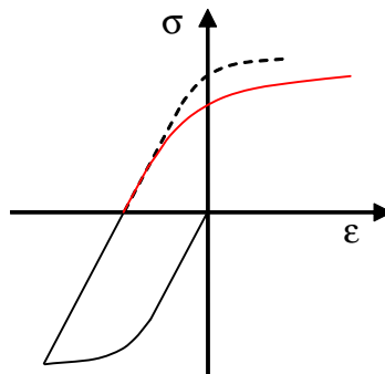
Figure 6 The Bauschinger effect is a phenomenon which occurs when materials are strained into the non-linear stress-strain area in one direction followed by straining in the opposite direction. The effect of such cycling is that the reversed yield stress is decreased
