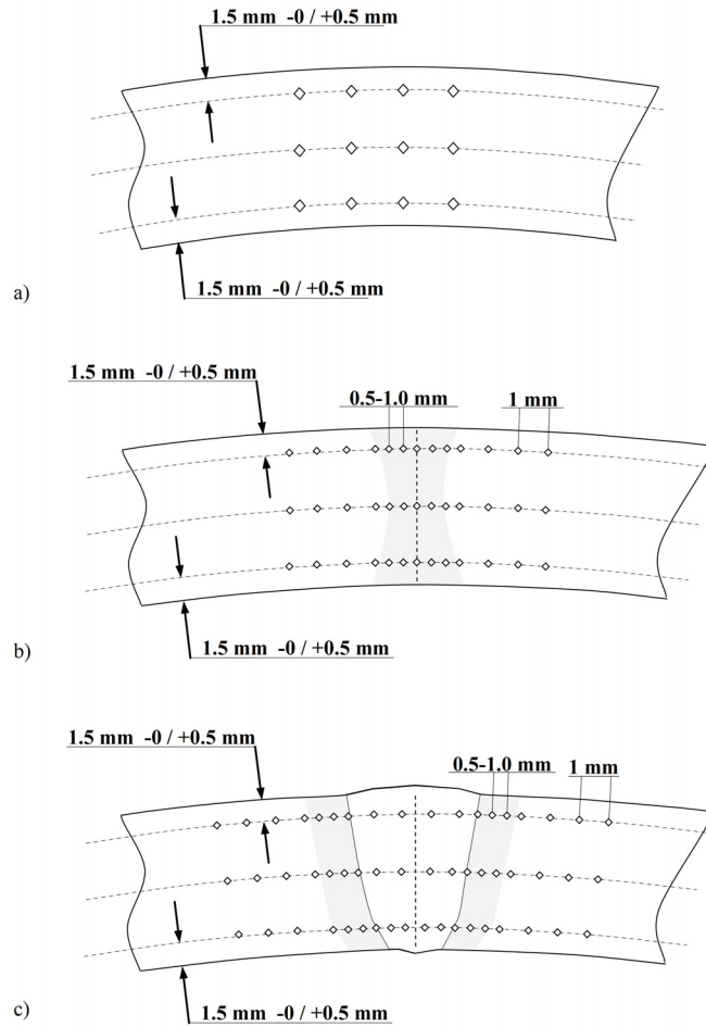
Figure 10 Hardness locations in a) seamless pipes, b) HFW pipe, and c) fusion welded joints.
