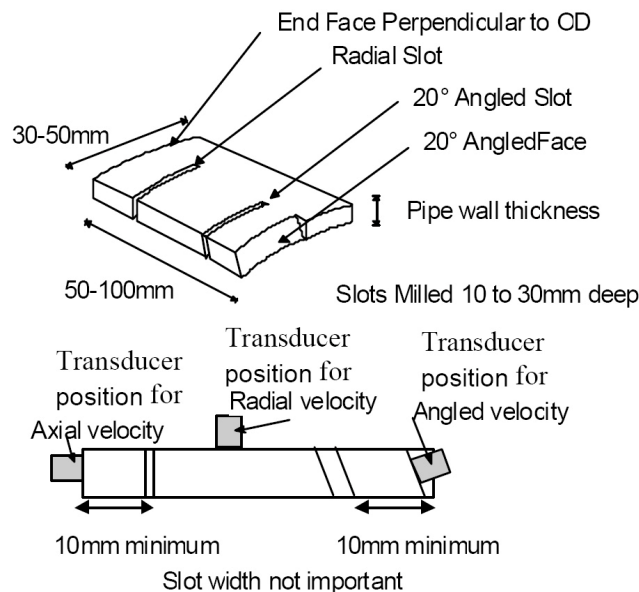
Figure 1 Test specimen and transducer placement
