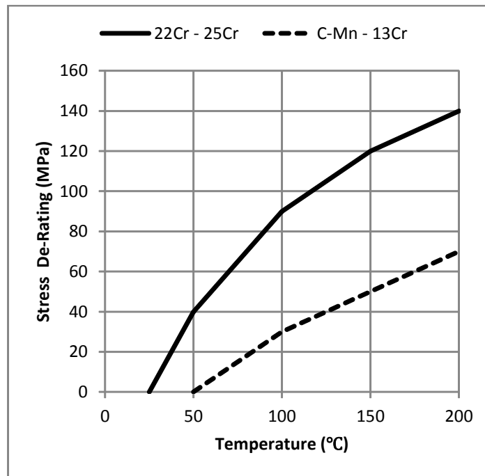
Figure 2 Proposed de-rating values for yield stress of C-Mn, 13Cr, 22Cr and 25Cr
