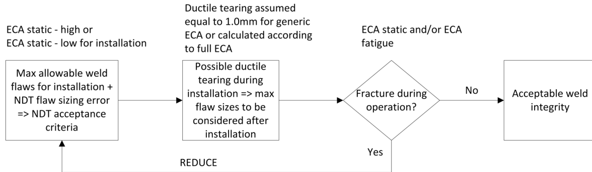
Figure 2 Illustration of a typical ECA process
