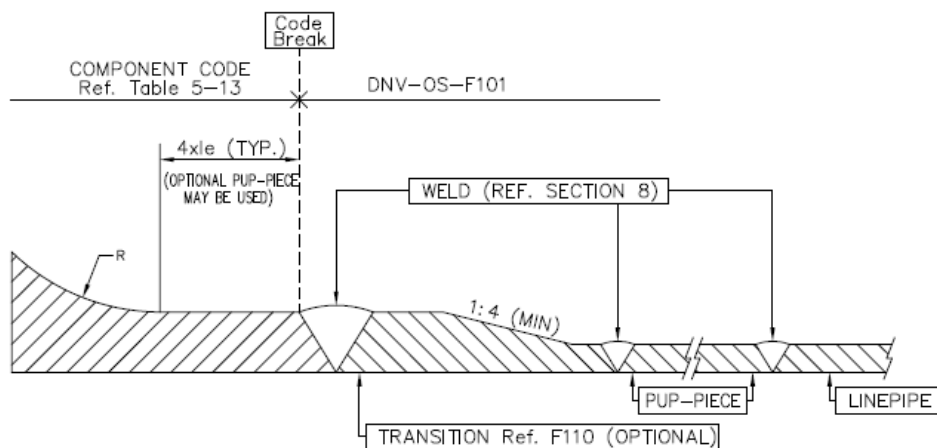
Figure 4 Code breaks between the line pipe and component connection
