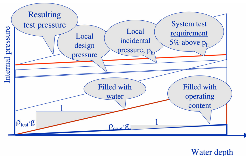
Figure 1 Illustration of local pressures and requirements to system pressure test
