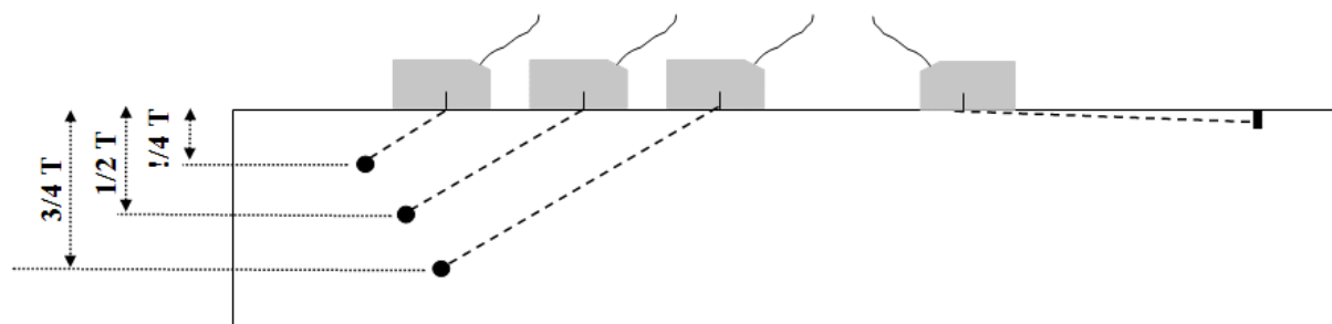
Figure 4 Reference block for construction of DAC, duplex stainless steel
