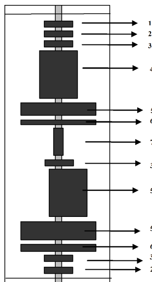
Figure 1 Welding procedure qualification test - sampling of test specimens for longitudinal butt welds.
