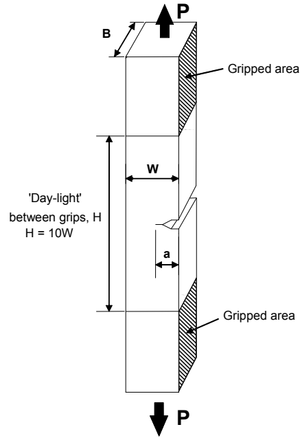
Figure 12 The clamped SENT (Single Edge Notched Tension) specimen
