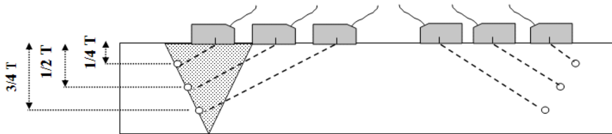
Figure 2 Reference block for construction of DAC, dimensions
