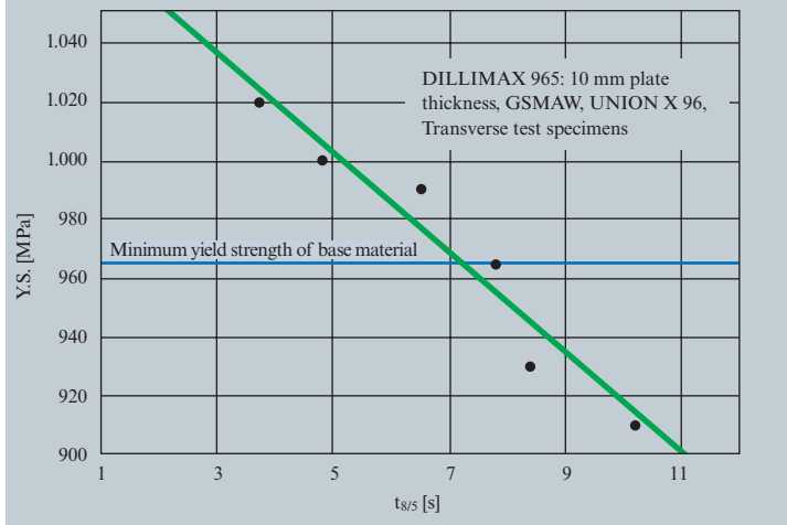
Figure 11: Effects of the t_{8/5} time on the yield strength of the weld metal of DILLIMAX 965
