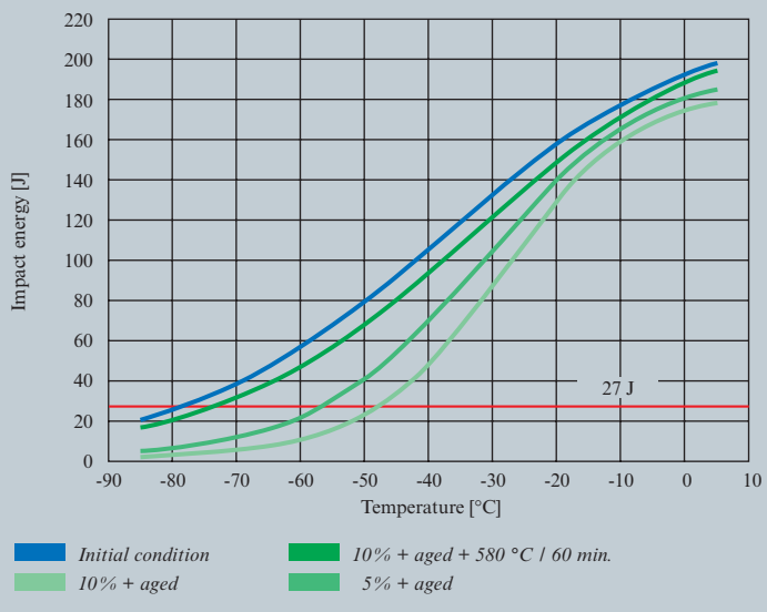
Figure 7: Effect of cold forming, ageing and stress relieving on the Charpy impact transition curves of DILLIMAX 690 T grade (plate thickness 30 mm)
