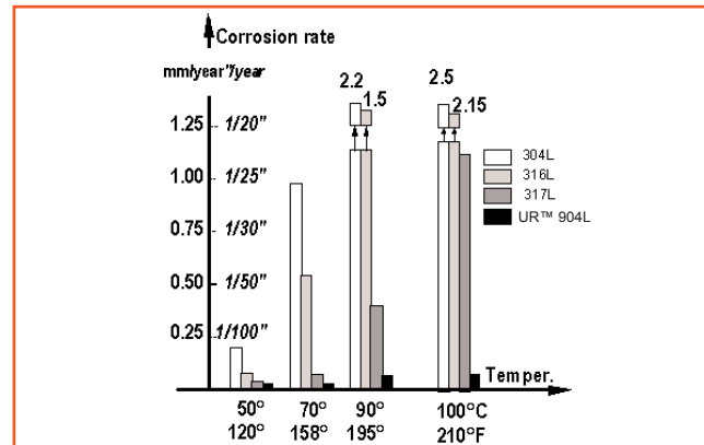
Corrosion rate of different types of stainless steels in industrial phosphoric acid (P2O5=48%, SO3=2.7%, F= 0.44%)
