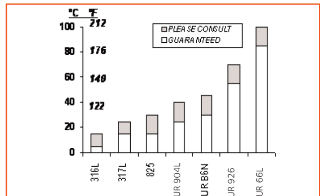
ASTM G48A - PITTING in Fe Cl 3 solution
