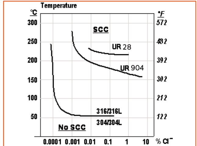
Practical experience and laboratory results of SCC in stainless steels
