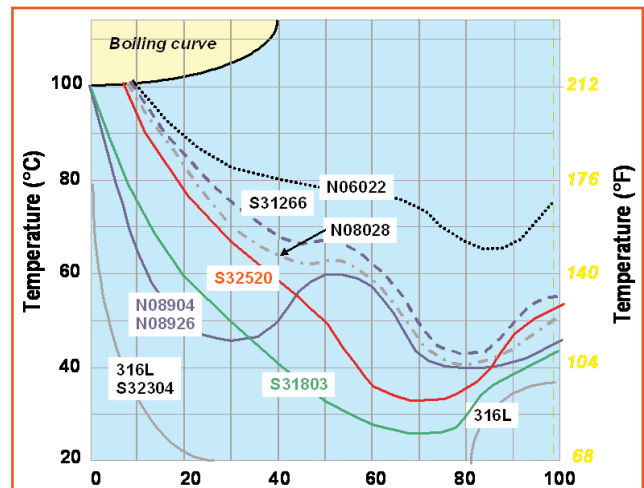
ISO – Corrosion diagram in industrial H 2 SO 4 (0,2mm/y)
