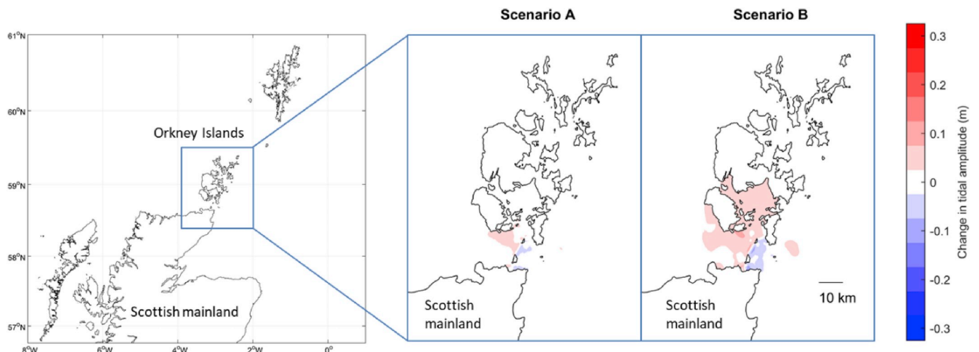
Fig. 2. Predicted changes to semi-diurnal tidal amplitude resulting from two turbine layouts which both extract a mean power of 1.4 GW. Figure adapted from O'Hara Murray and Gallego [20].
