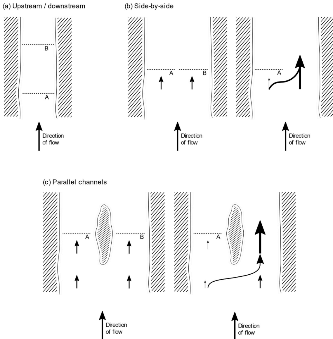
Fig. 3. Three idealised scenarios showing interactions between two tidal farms A and B. In scenarios (b) and (c), we also show the effect of farm B being absent or inoperative.
