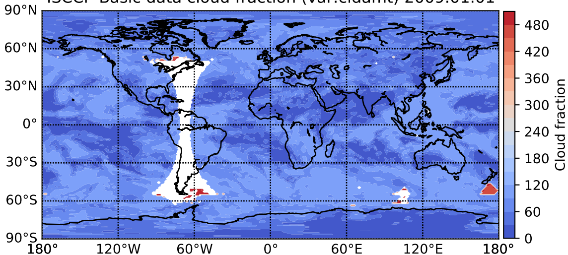
ISCCP-Basic data cloud fraction (var:cldamt) 2009.01.01
