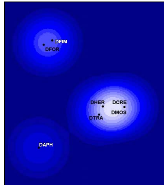
Fig. 12. Clusters of Dendrobium species, obtained by using kernels on the CCA scores.
