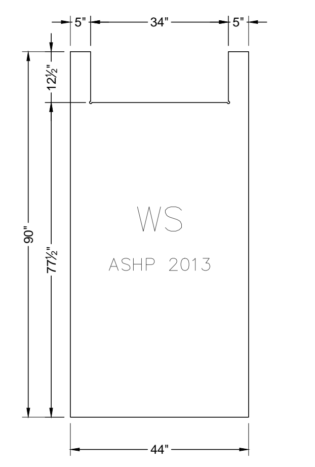
BASEPLATE JIG - WS SCALE: 1/2" = 1'-0" (6 REQ'D)
