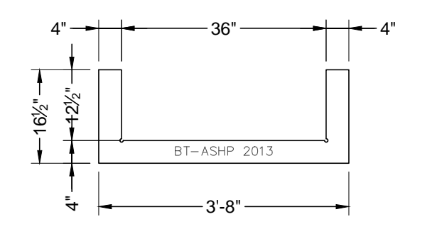
BASEPLATE JIG - BT SCALE: 1/2" = 1'-0" (1 REQ'D)
