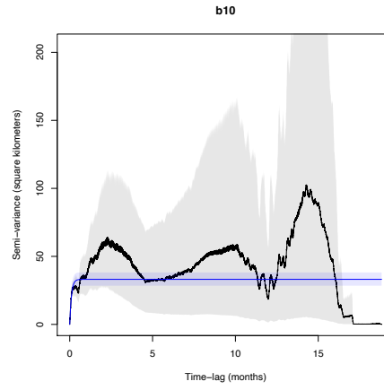
Variogram with all points
