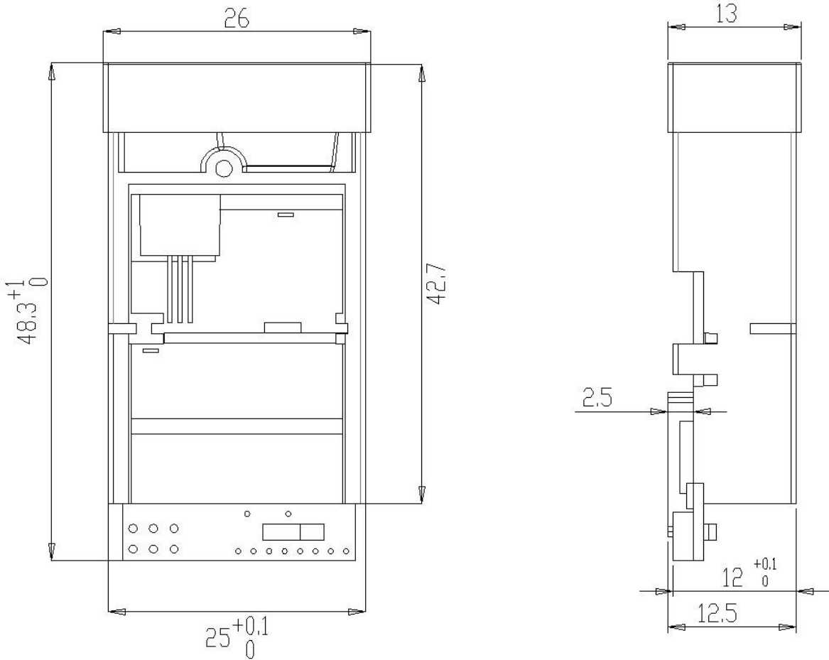
Figure 3-1 Mechanical Size
