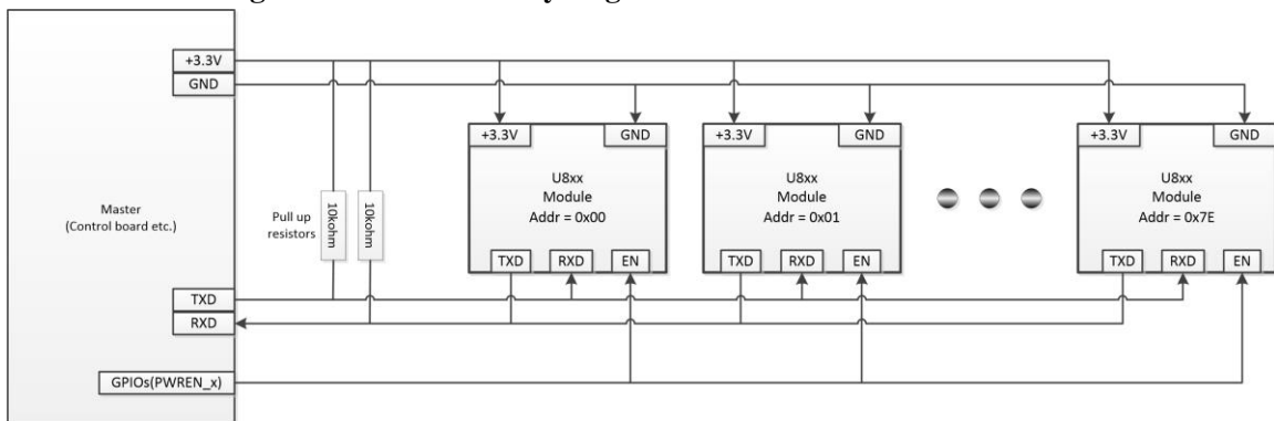
Figure 4-1 Multi-Module Wiring
