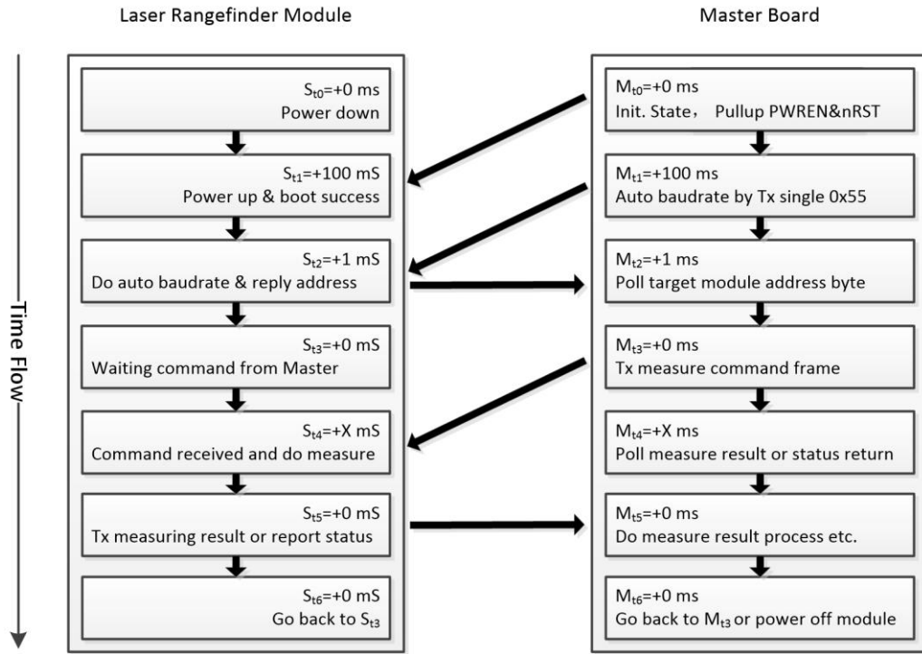
Figure 6-1 Control Flow
