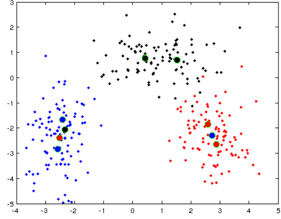
2) Adapting the UBM to each class
